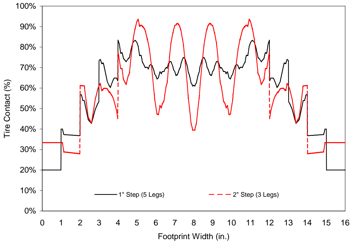
FIGURE 10 Comparative amount of tire-pavement contact as measured along the test width during uni-directional loading mode with a 4-inch wheel wander, in 1- and 2-inch increments respectively.
